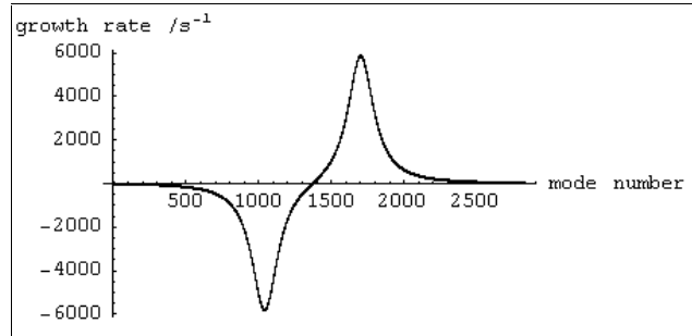
Figure 5: Coupled bunch growth rates in the TESLA damping ring.
