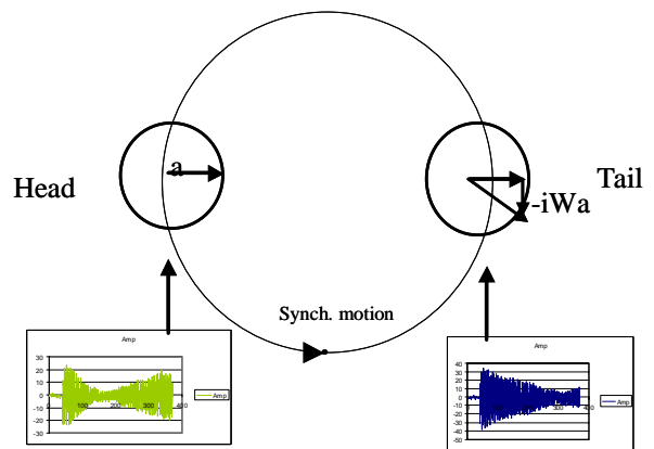
Fig. 8: The wake field W creates a phase advance for the tail depending on the position of the head. Following the phase evolution of head and tail over a synchrotron period can give details about W .
